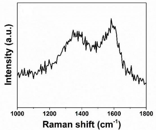
Figure 2: Raman spectra of the sample
