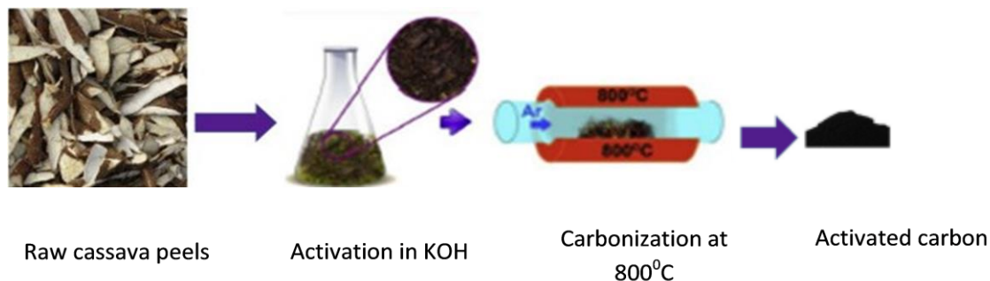
Scheme 1: Production of activated carbon from cassava peels
